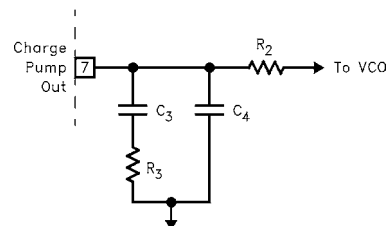
FIGURE 7. TYPICAL LOOP FILTER
